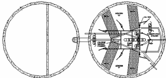
SEPTIC TANK
