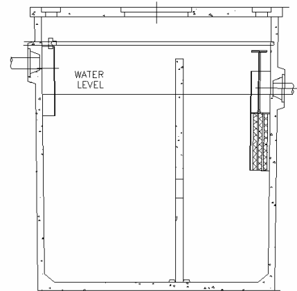
ELEVATION (with lid)
